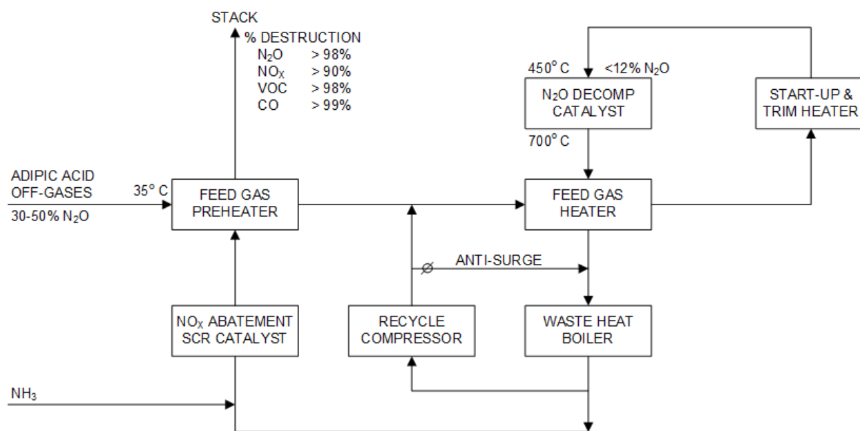
Figure 2.2. Typical Process Flowsheet for Catalytic Decomposition of \text{N}_2\text{O}
